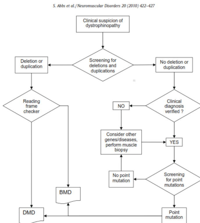
Fig. 1. Flow chart for the diagnostic work-up of a dystrophinopathy.
